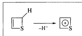
Scheme 8.16
