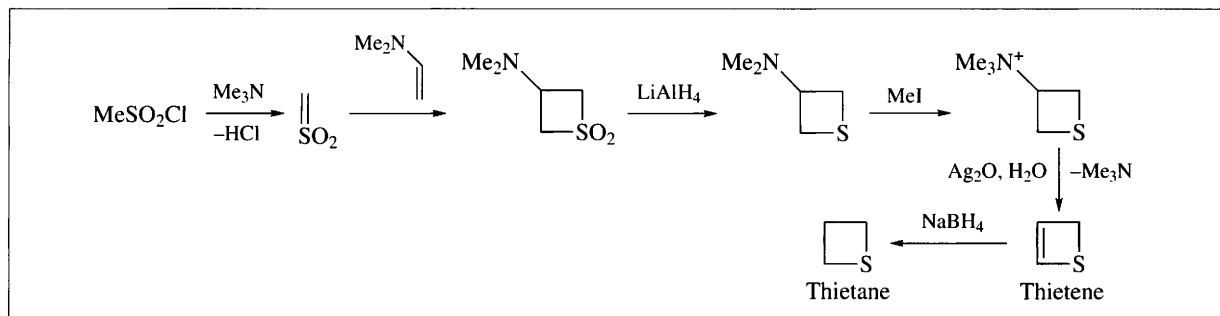
Scheme 8.15
