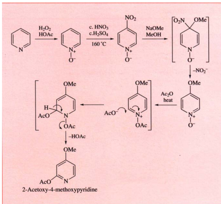
Scheme 2.15
