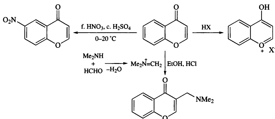
Scheme 5.7
