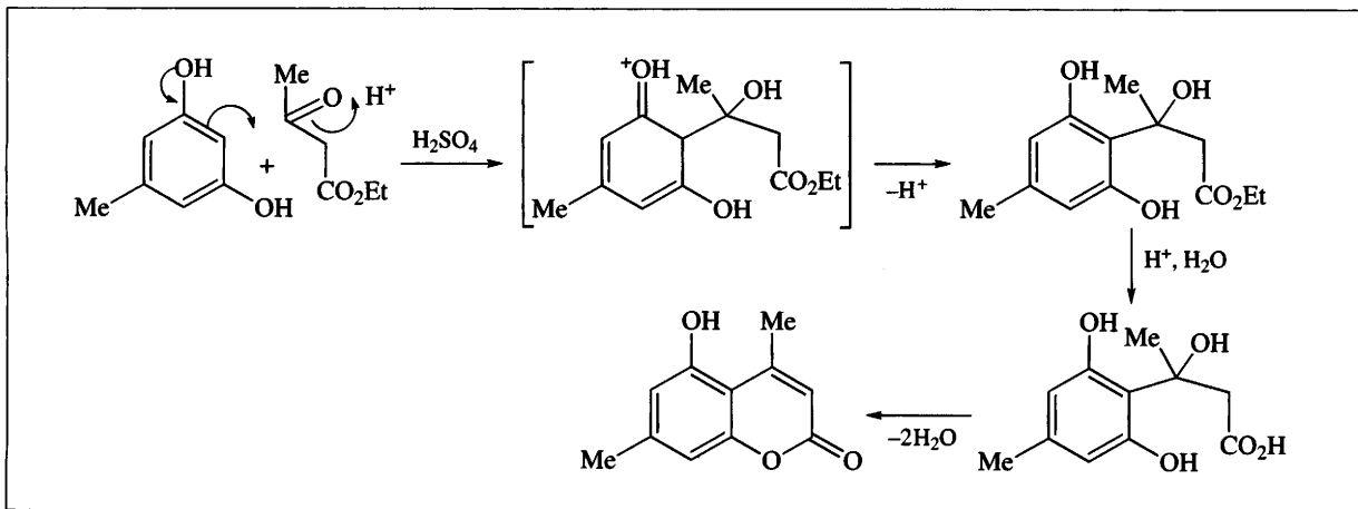
Scheme 5.6
