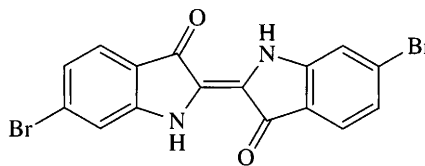
7.7 Tyrian purple
