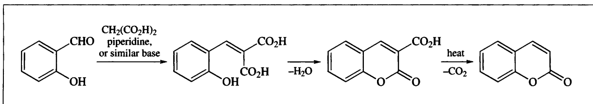
Scheme 5.5
