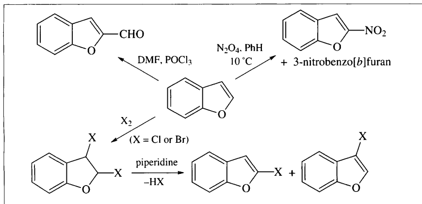
Scheme 7.21
