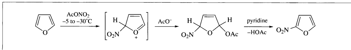
Scheme 6.22
