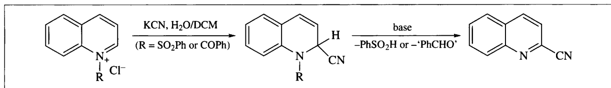
Scheme 3.5
