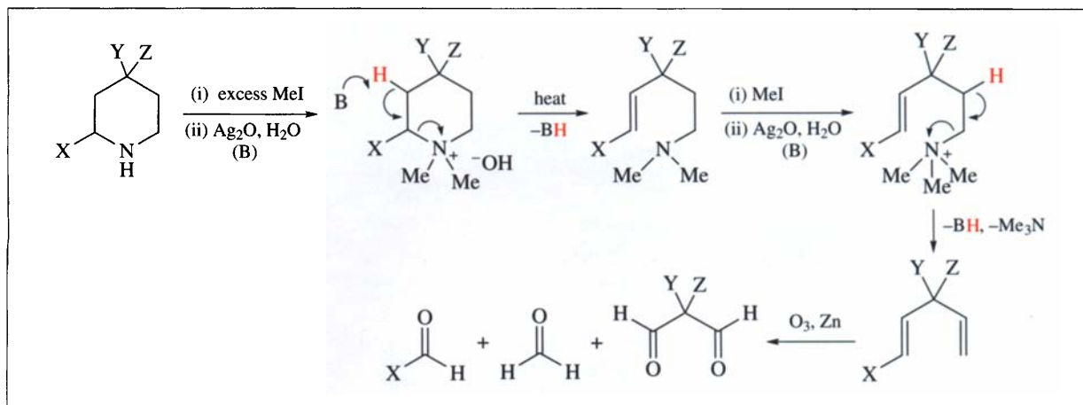
Scheme 2.32
