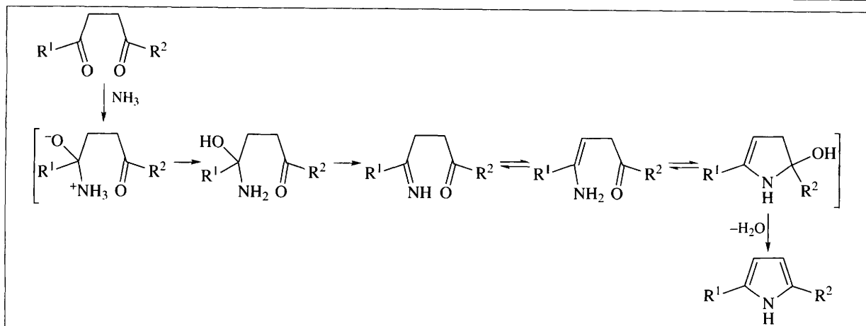
Scheme 6.13
