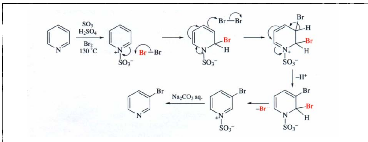
Scheme 2.4
