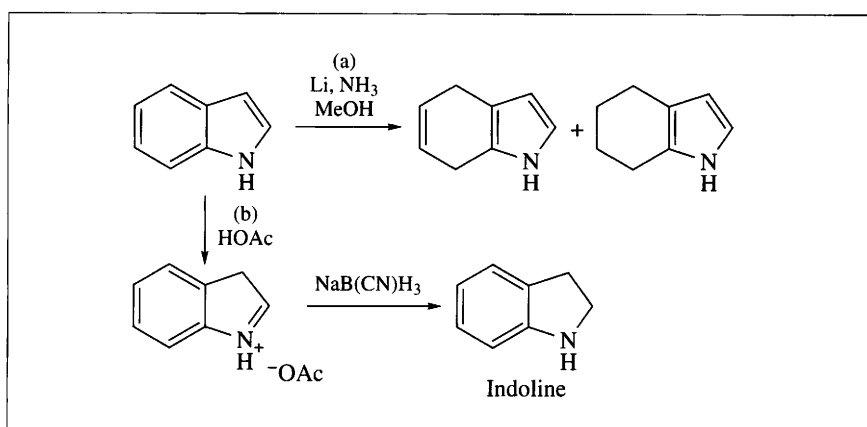
Scheme 7.13
