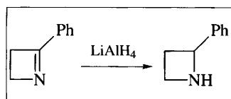
Scheme 8.3
