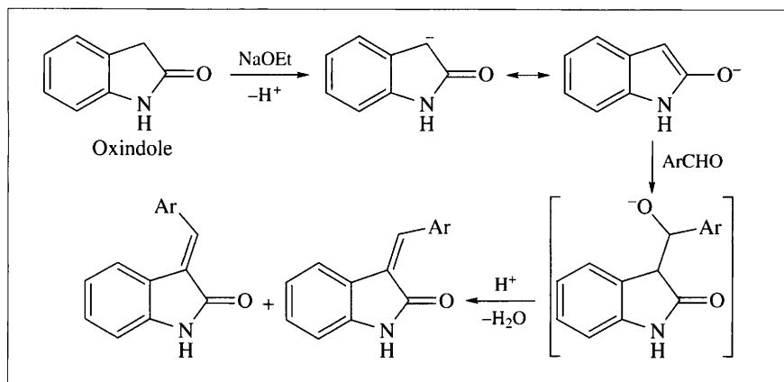
Scheme 7.20
