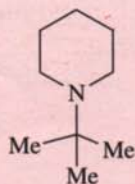
1- tert -Butylpiperidine
