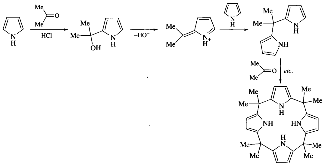
Scheme 6.7
