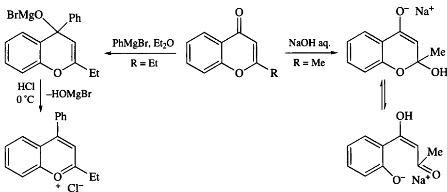
Scheme 5.8
