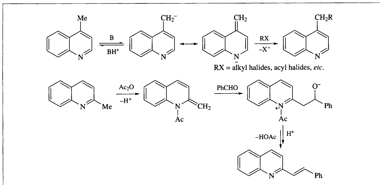
Scheme 3.9
