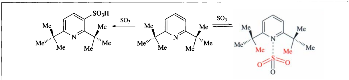
Scheme 2.3
