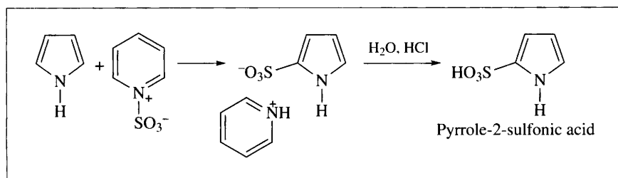
Scheme 6.3
