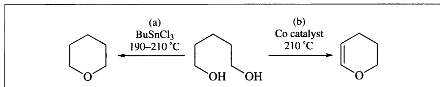
Scheme 4.12
