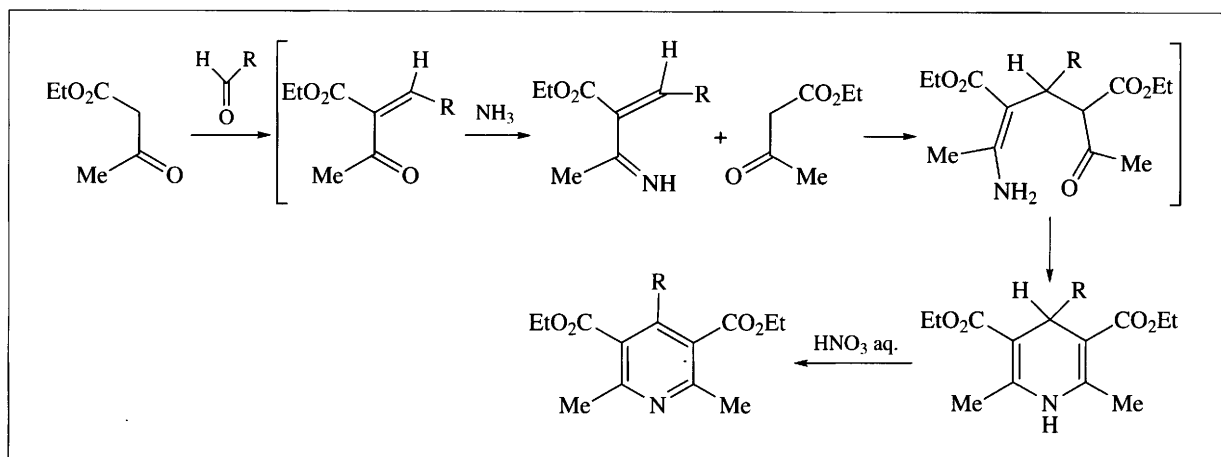
Scheme 2.18
