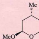
trans -2-Methoxy-4-methyltetrahydropyran
