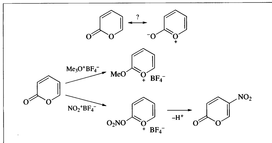
Scheme 4.5
