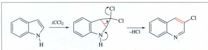
Scheme 7.12
