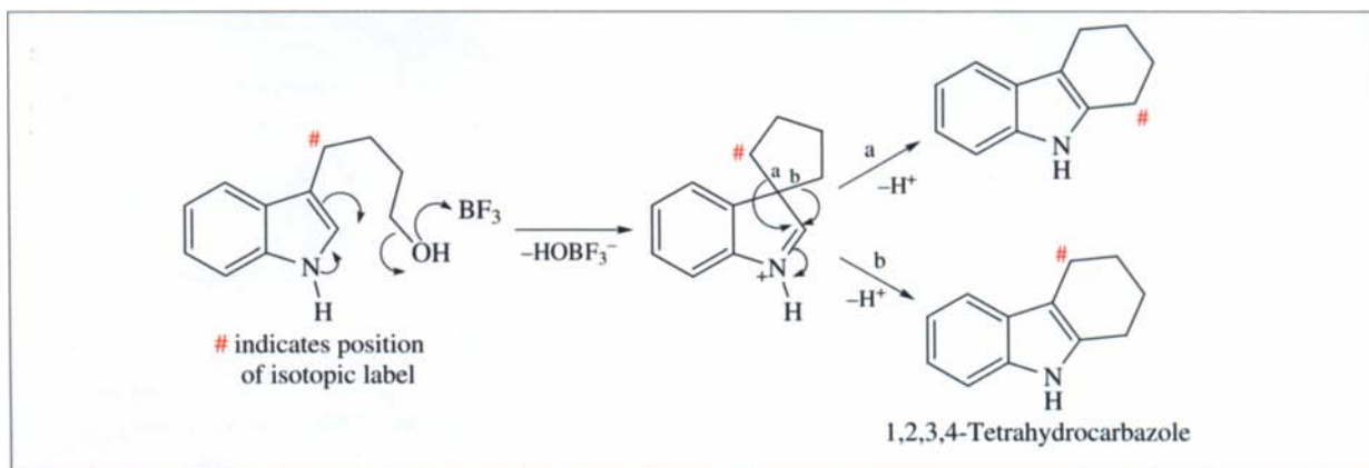
Scheme 7.3
