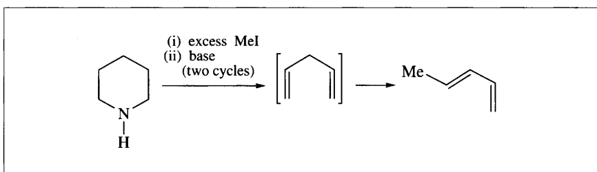
Scheme 2.33
