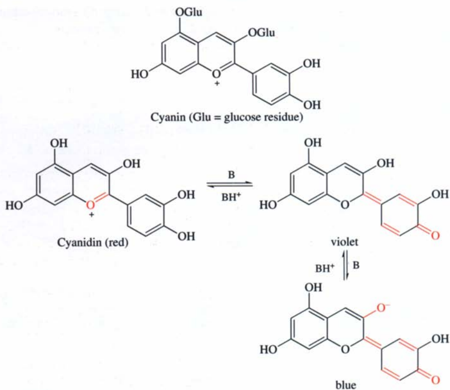
Scheme 5.1
