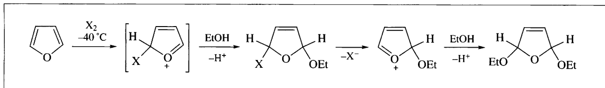
Scheme 6.23
