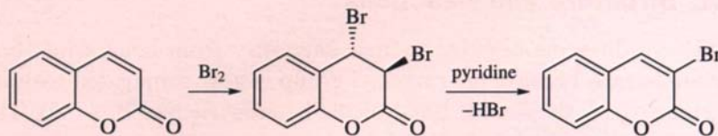
Scheme 5.4
