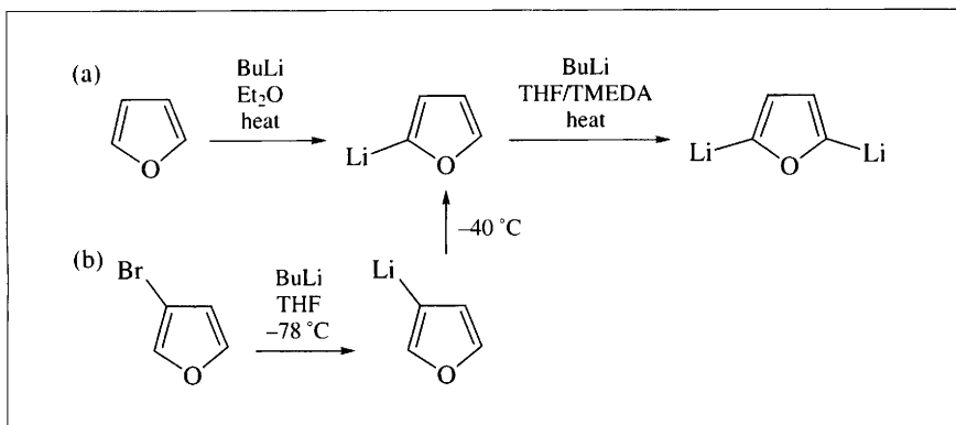
Scheme 6.26
