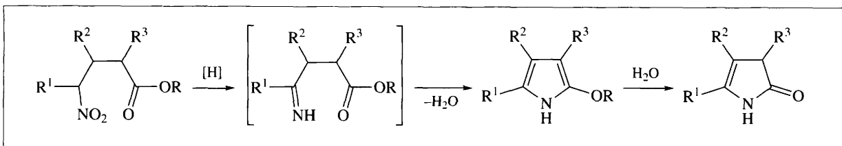
Scheme 6.15
