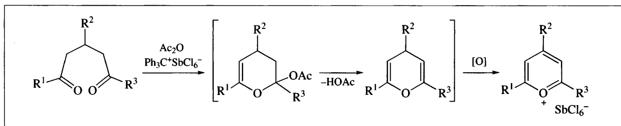
Scheme 4.4
