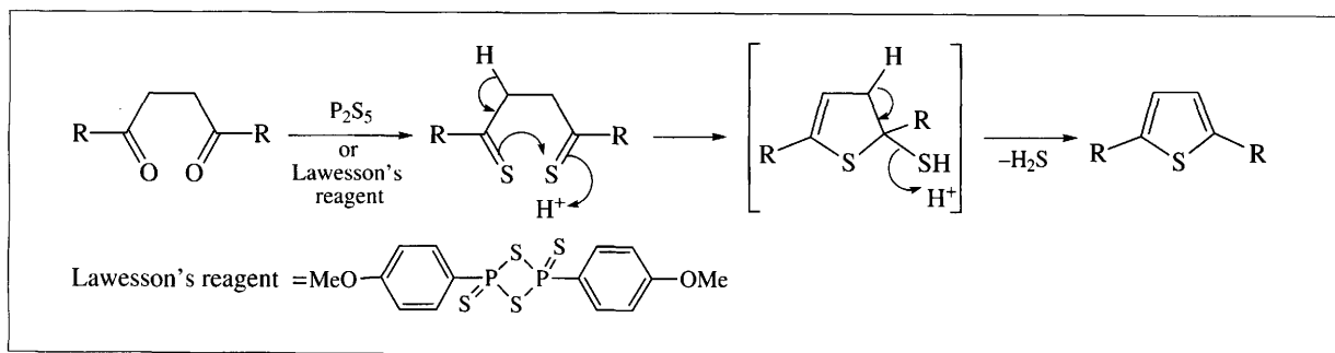
Scheme 6.37
