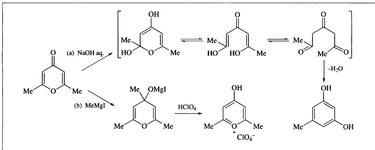
Scheme 4.11
