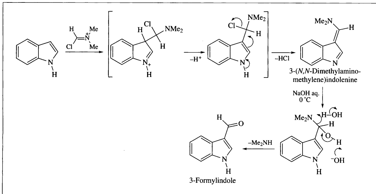
Scheme 7.5
