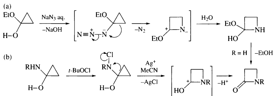
Scheme 8.7
