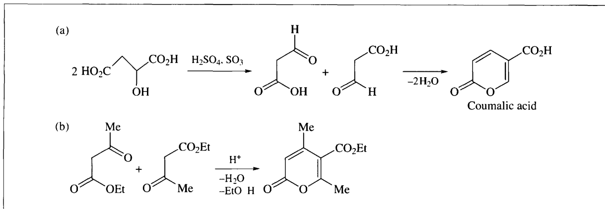
Scheme 4.8
