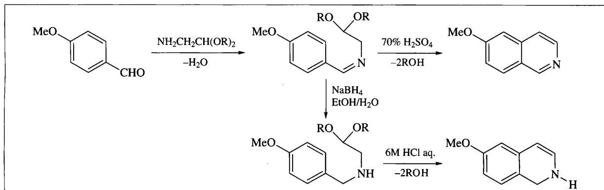
Scheme 3.20
