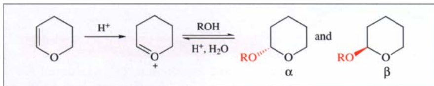
Scheme 4.13
