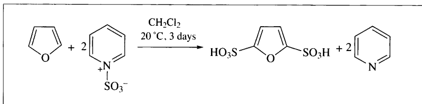
Scheme 6.24
