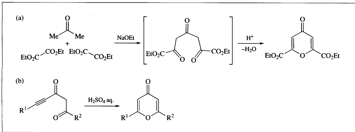
Scheme 4.11
