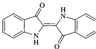
7.6 Indigotin (indigo)
